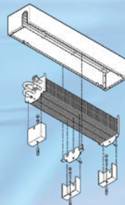
Scope of delivery Hood convector with console for finished floor
